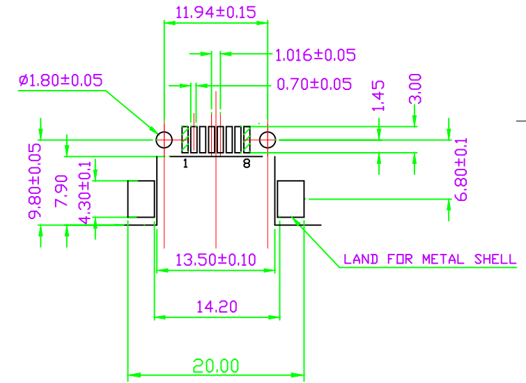
PCB LAYOUT
